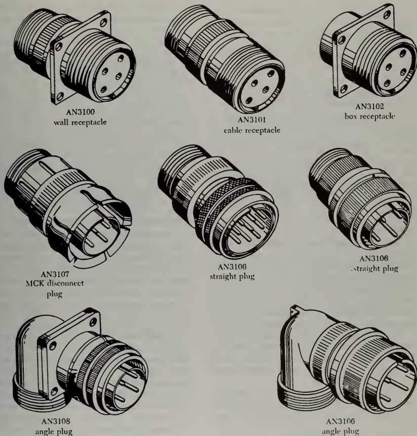
FIGURE 4-118. AN connectors.
